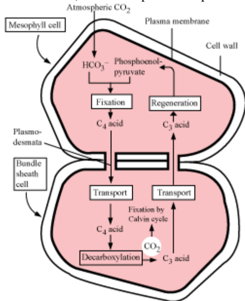
Hatch and Slack pathways
